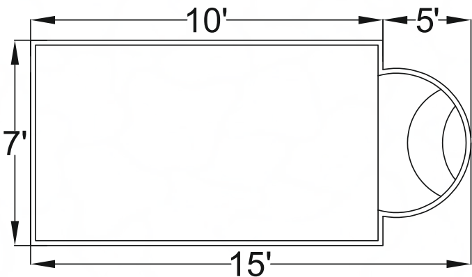
ROMAN SHAPED SWIMMING POOL - (15'X7'X4'.5") MODEL - MODEL - 1
